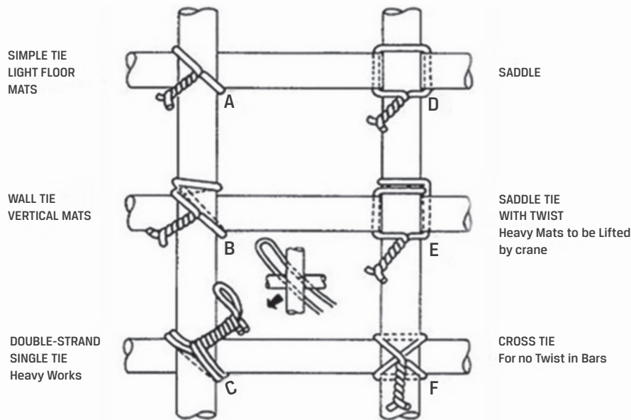
Figure: Six ways to tie rebar.
